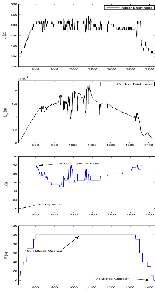
Figure 7. Evolution of indoor illuminance for a 24hour August simulation
