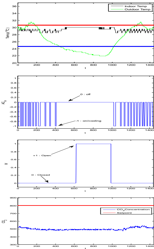
Figure 3. Evolution of indoor temperature and indoor CO 2 concentration for a 24hour July simulation (N.V.B)
