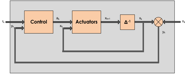
Figure 1. The control system diagram
