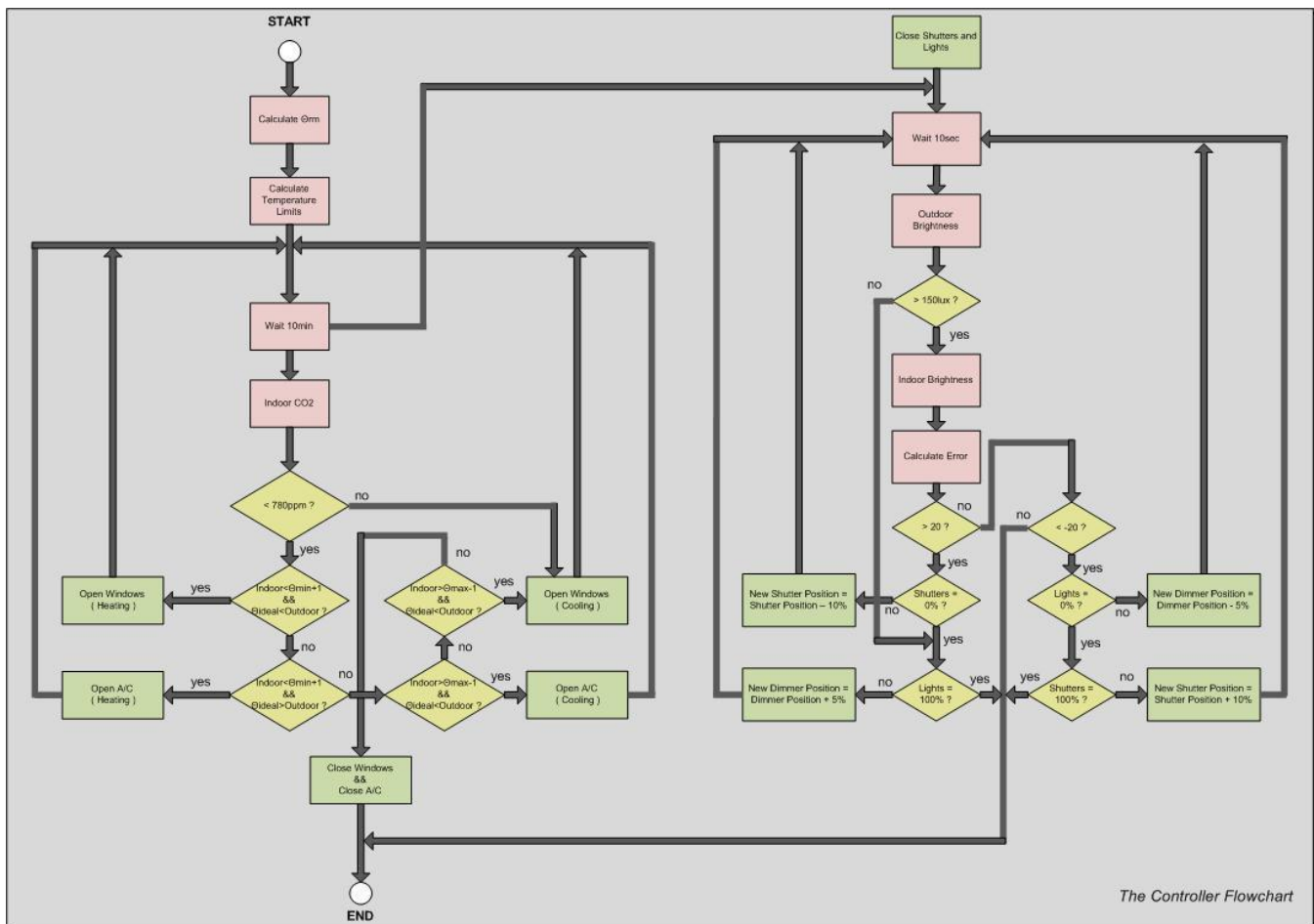
Figure 2. The Control Algorithm
