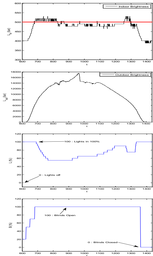
Figure 6. Evolution of indoor illuminance for a 24hour July simulation
