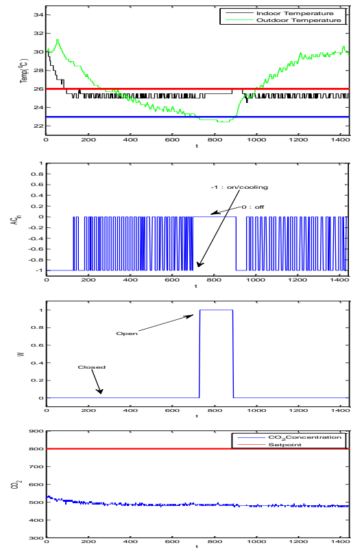
Figure 5. Evolution of indoor temperature and indoor CO 2 concentration for a 24hour August simulation (B.M.C/H)
